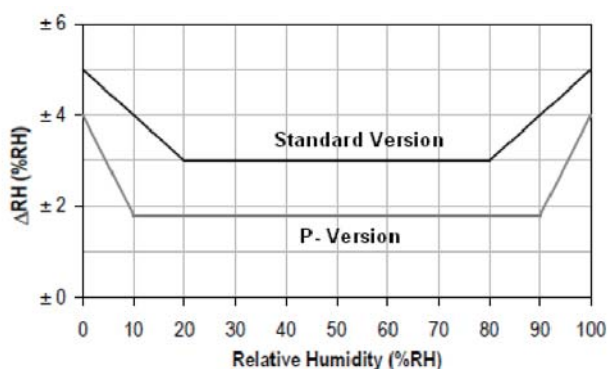
Maximum RH-tolerance at 25°C per sensor.
