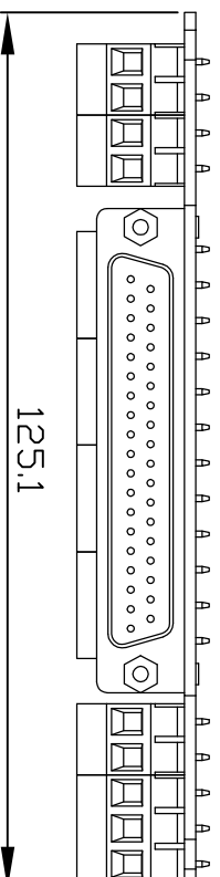
Top View
