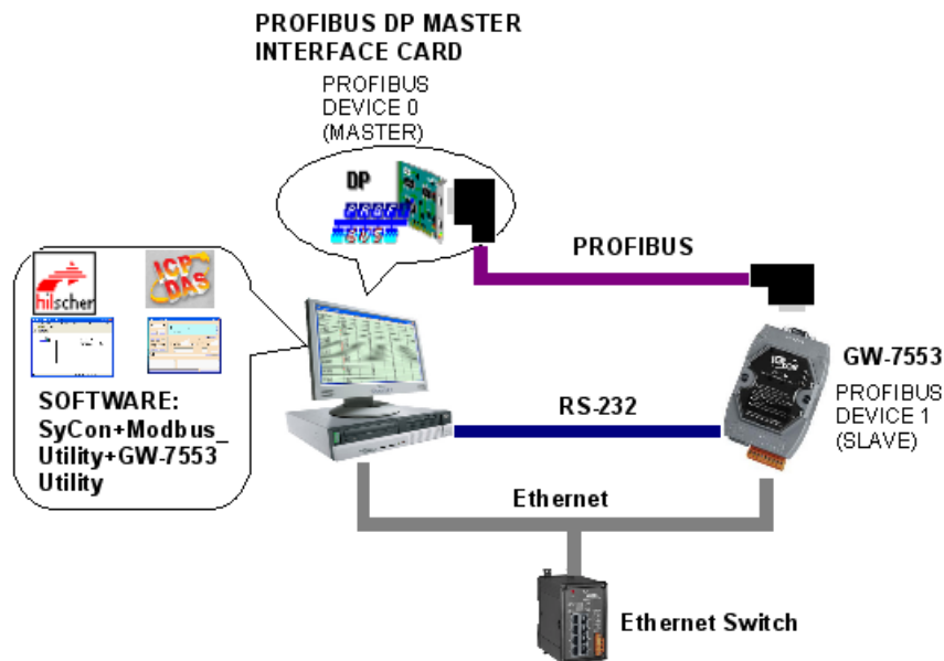
Application example of PROFIBUS to Modbus TCP
