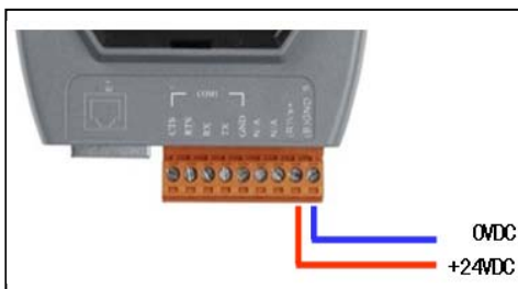
Power connection
